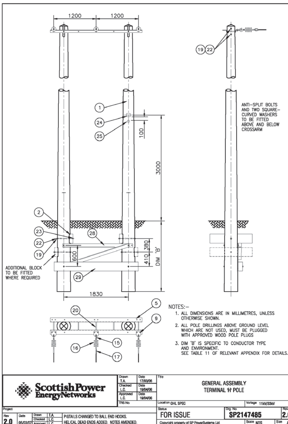
Figure 18 "H" Pole Terminal (Drawing 2147485)
